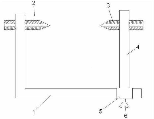
图 1 自制髂骨穿针导向器示意图 Fig.1 A schematic diagram of a self-made iliac needle guide
